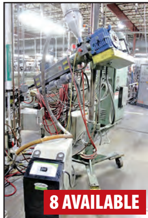
DAVIS STANDARD DS125 1.25" 24:1 CO-EXTRUDER
